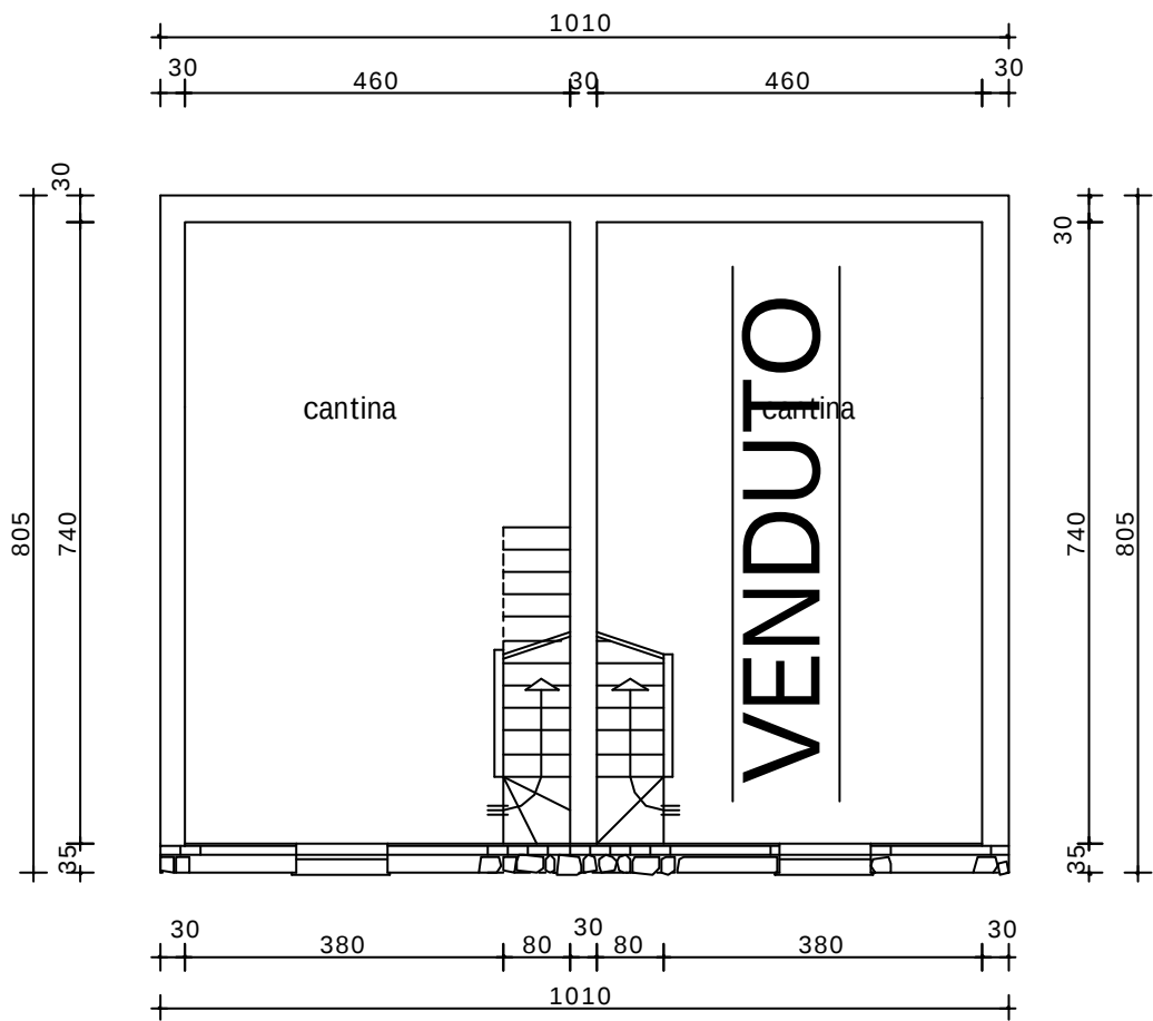
PIANO INTERRATO
